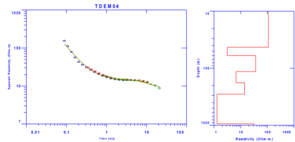
Figure 9. Inversion result for the central loop sounding TDEM04.
